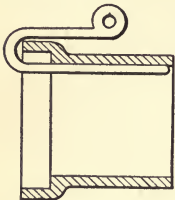
FIG. 19.—PIPE-LAYING HOOK.
